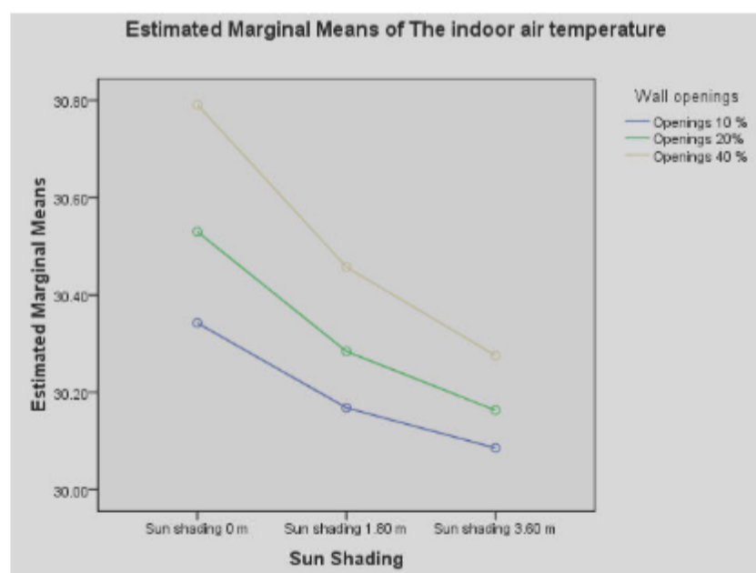
Figure-5. Interaction between width sun shading and wall openings to the indoor air temperature.
