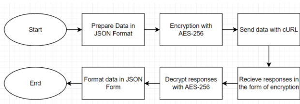
Figure 10. QRIS Flowchart
