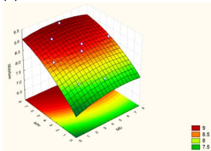
Gambar 5. Grafik Fitted Surface Kadar Air
