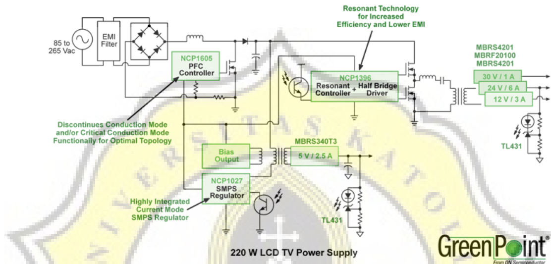
Gambar B.1. Catu Daya Monitor LCD
