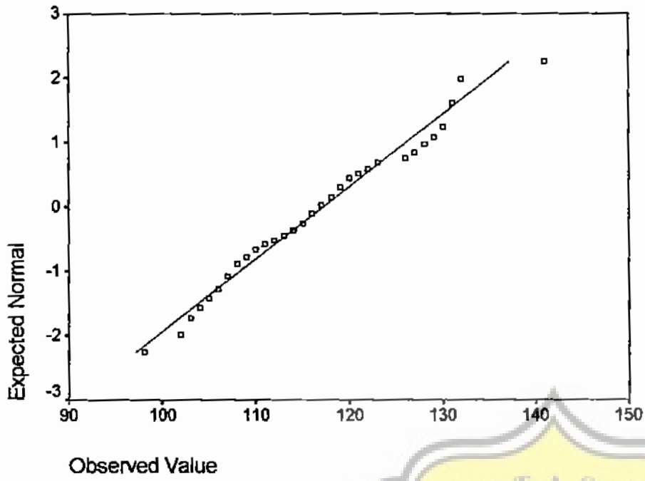
Normal Q-Q Plot of Asertivitas
