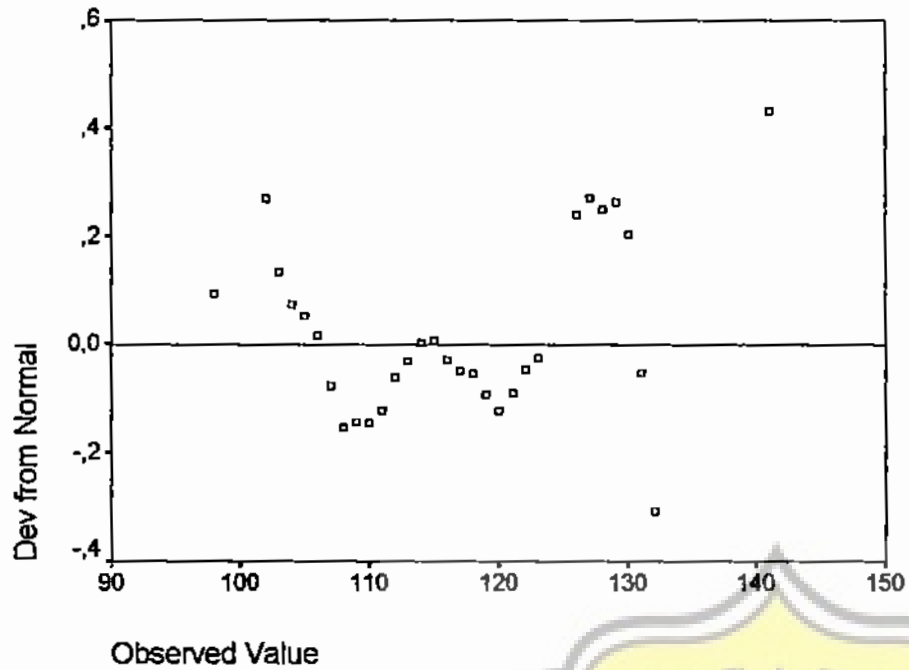
Detrended Normal Q-Q Plot of Asertivitas
