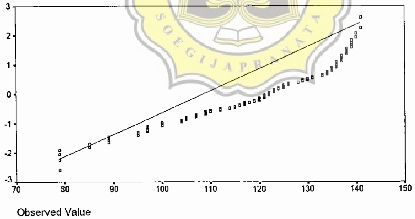
Normal Q-Q Plot of Y PERSEPSI TERHADAP AIDS
