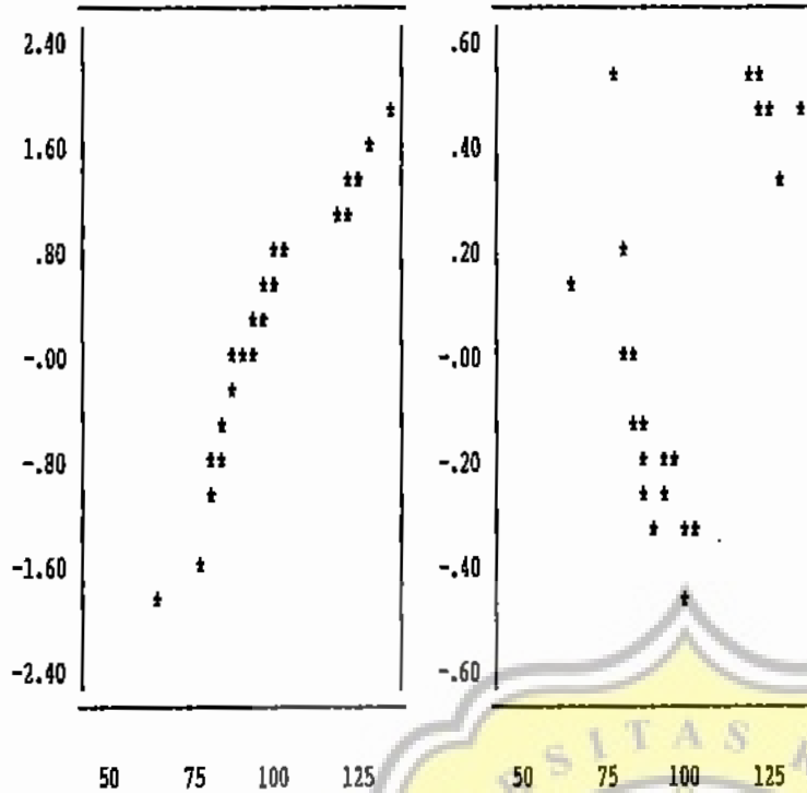
Normal Plot
