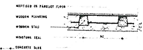
Typical floor construction
