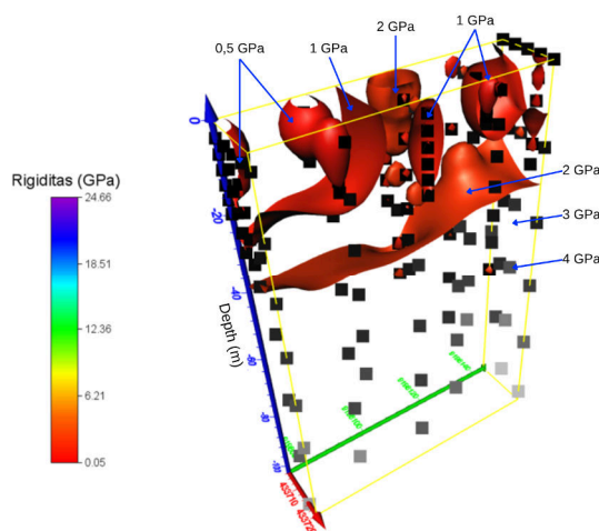
Figure 10. Rigidity of the soil layer in GMKA based on the GPR test
