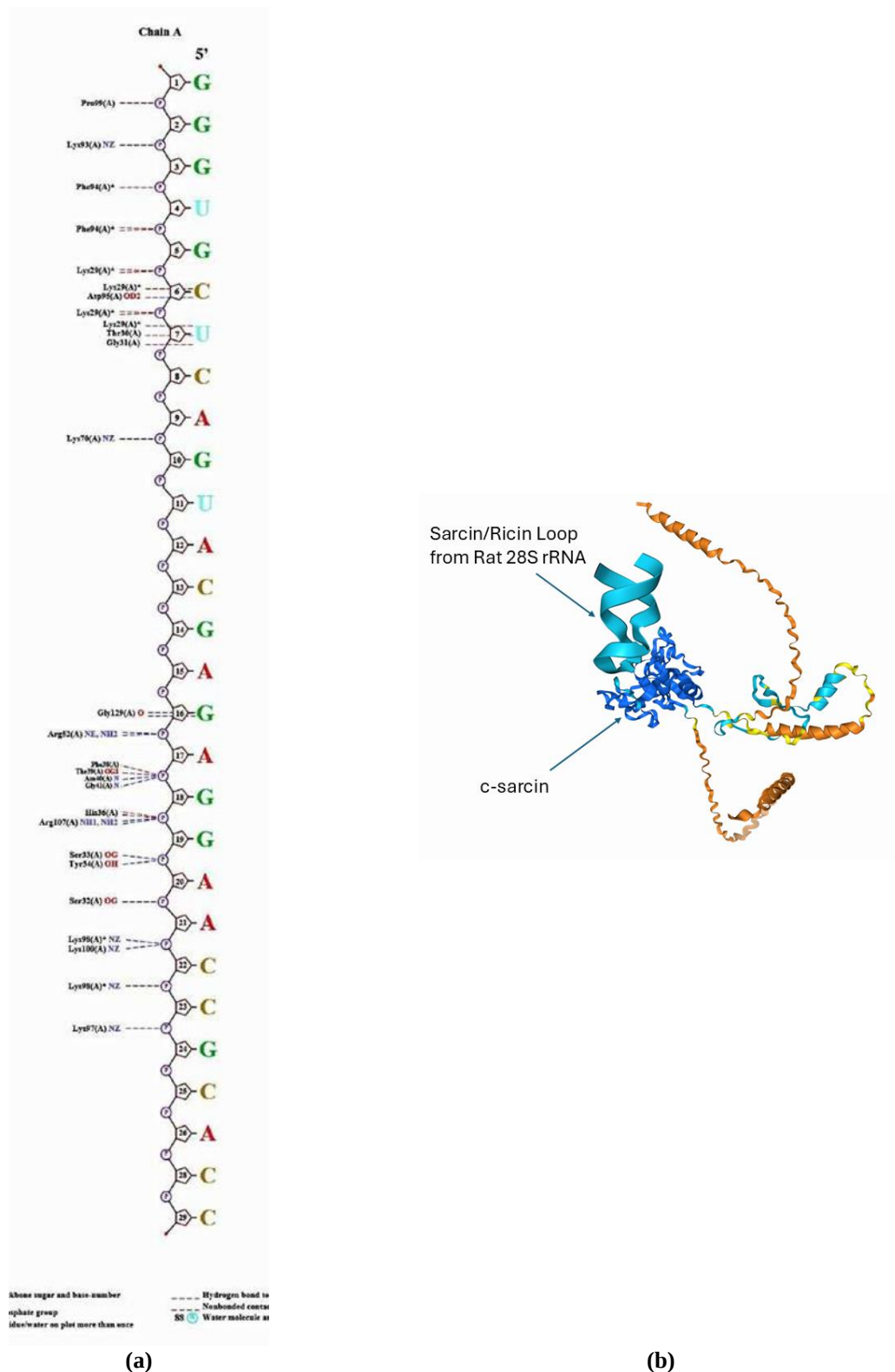
Figure 5. (a) The interaction between the rat 28S rRNA sarcin/ricin loop with ribotoxin \alpha -sarcin; (b) Three-dimensional structure binding between the rat 28S rRNA sarcin/ricin loop with c-sarcin.
