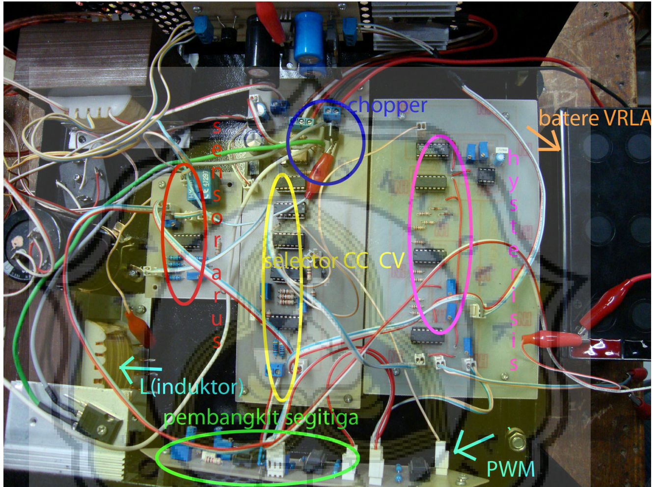
Gb. Prototip Rangkaian Pengisian Batere VRLA Metode Constan Current Constan Tegangan (CC CV)
