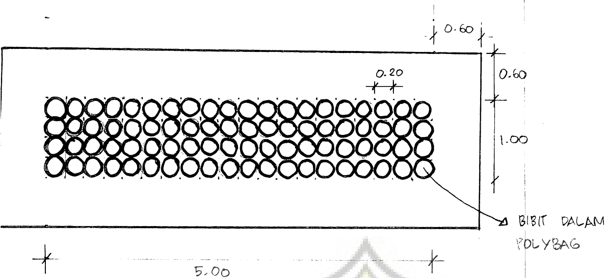
LAY OUT PENANAMAN TANAMAN HIAS : PALEM.
