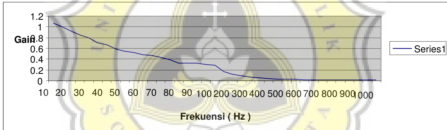
Gambar 4.1 Kurva Pengujian Low Pass Filter
