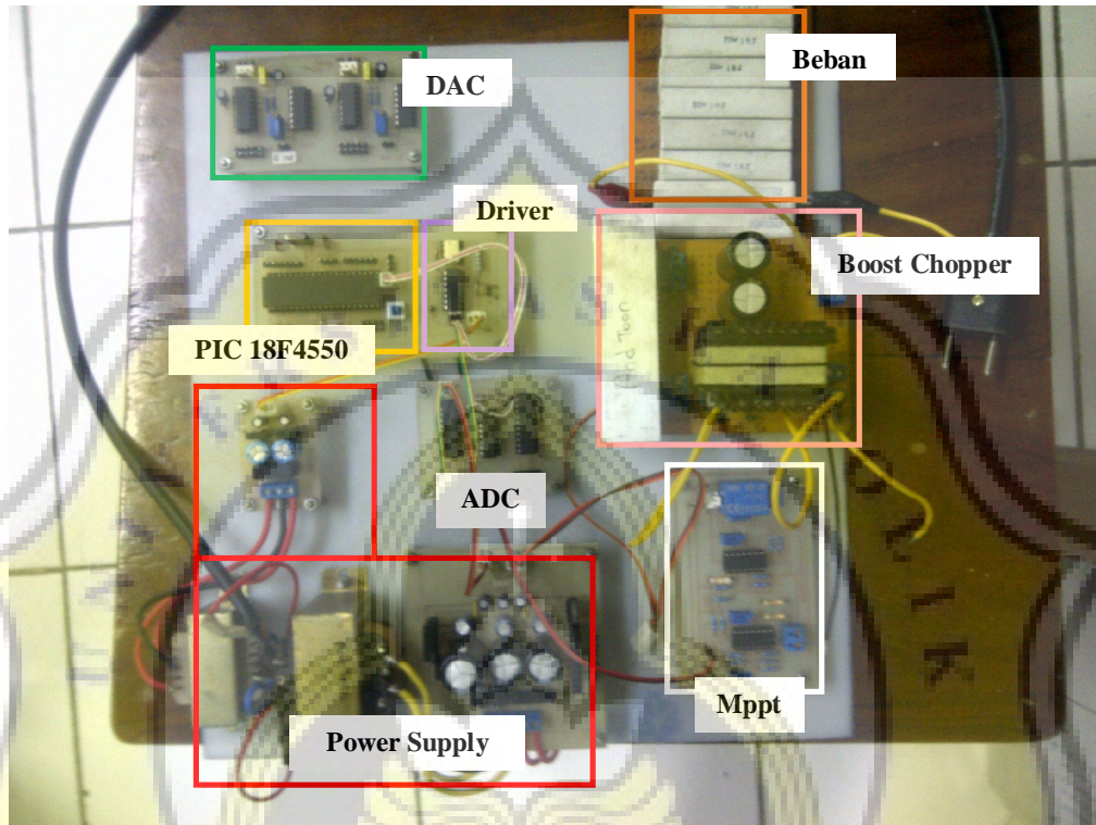
Gambar 1 Realisai alat
