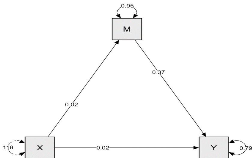
Gambar 2. Path Plot
