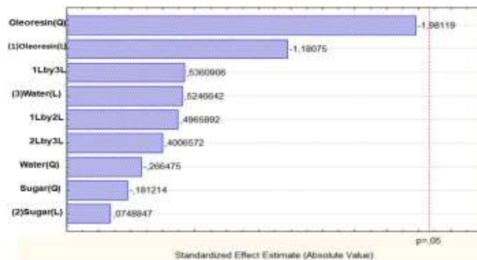
Figure 1. Pareto Chart of Water Content Standardized Effects
