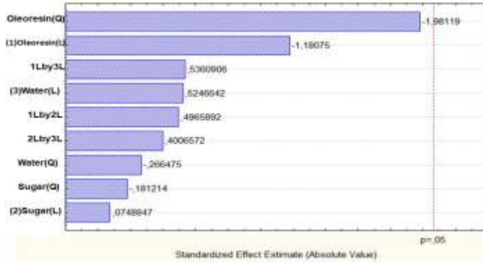
Fig. 5. Pareto Chart of Water Content Standardized Effects
