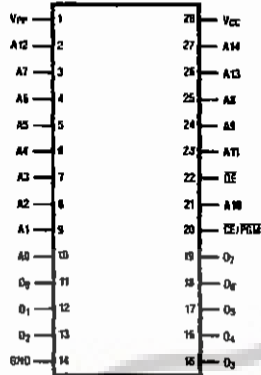
27C256Q Dual-In-Line Package
