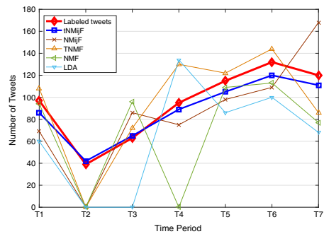
(c) Tweet distributions over time periods for the topic MB180 with different topic derivation methods
