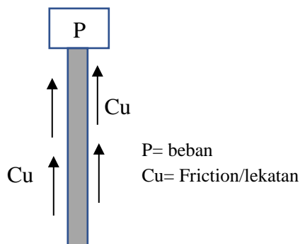
Gambar 3. 1. Konsep Floating pile
