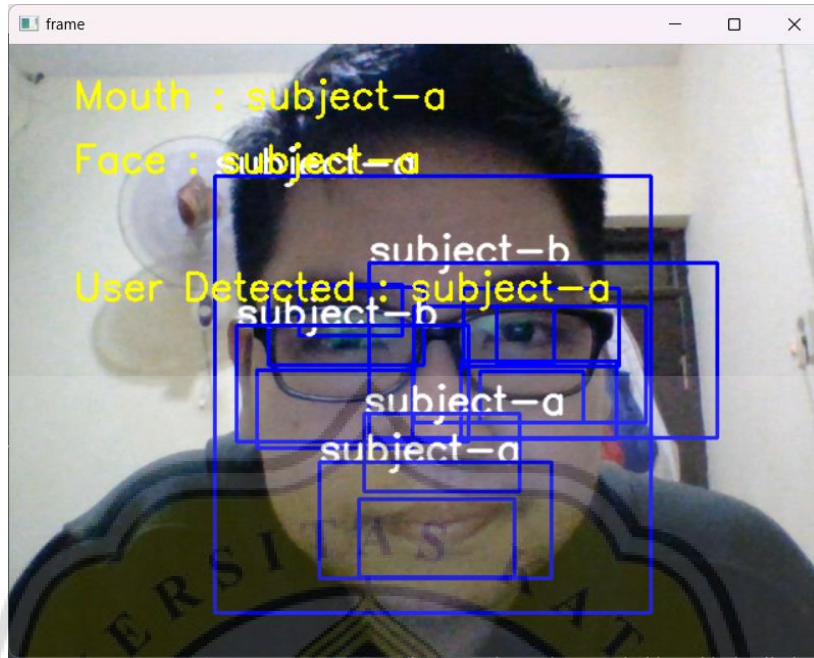
Figure 6.12 Glasses Result
