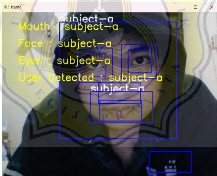
Figure 6.11 Hoodie Result
