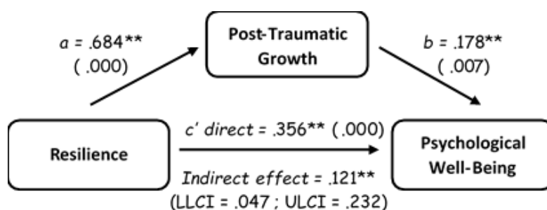
Path Analysis Result
