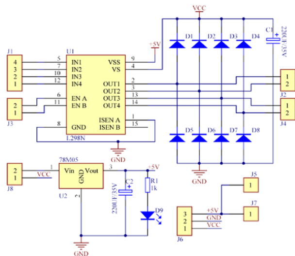
Gambar 3. Skematik motor driver L298N
