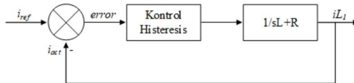
Gambar 5. Diagram Blok Sistem Kendali Arus Histeresis
