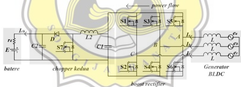
Gambar 3. Rangkaian Ekivalen Generator BLDC (Riyadi dkk., 2019)
