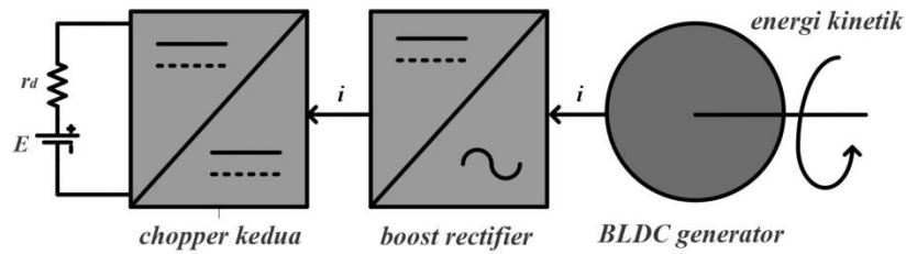
Gambar 1. Blok Diagram Generator BLDC (Riyadi dkk., 2019)
