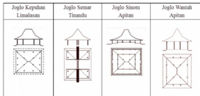
Gambar 2.11 Macam denah rumah Joglo Sumber: google.com. 2018
