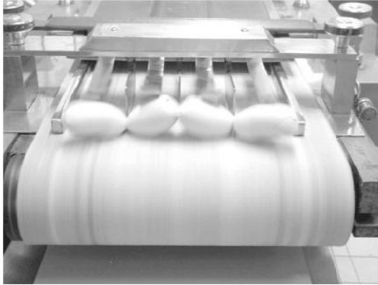
Figure 28.2 Final molder—four-piece. Courtesy of Campden BRI.
