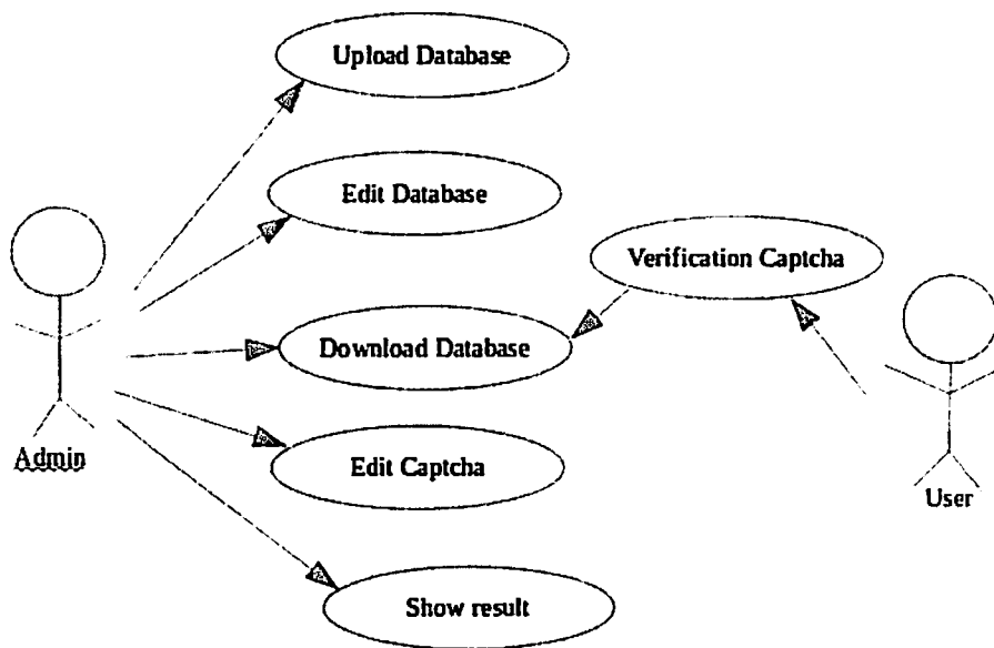
Fig. 4.1.1 Use Case Diagram
