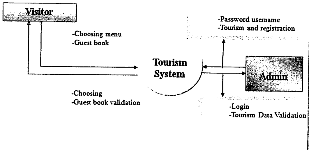
Figure 4.1 Context diagram
