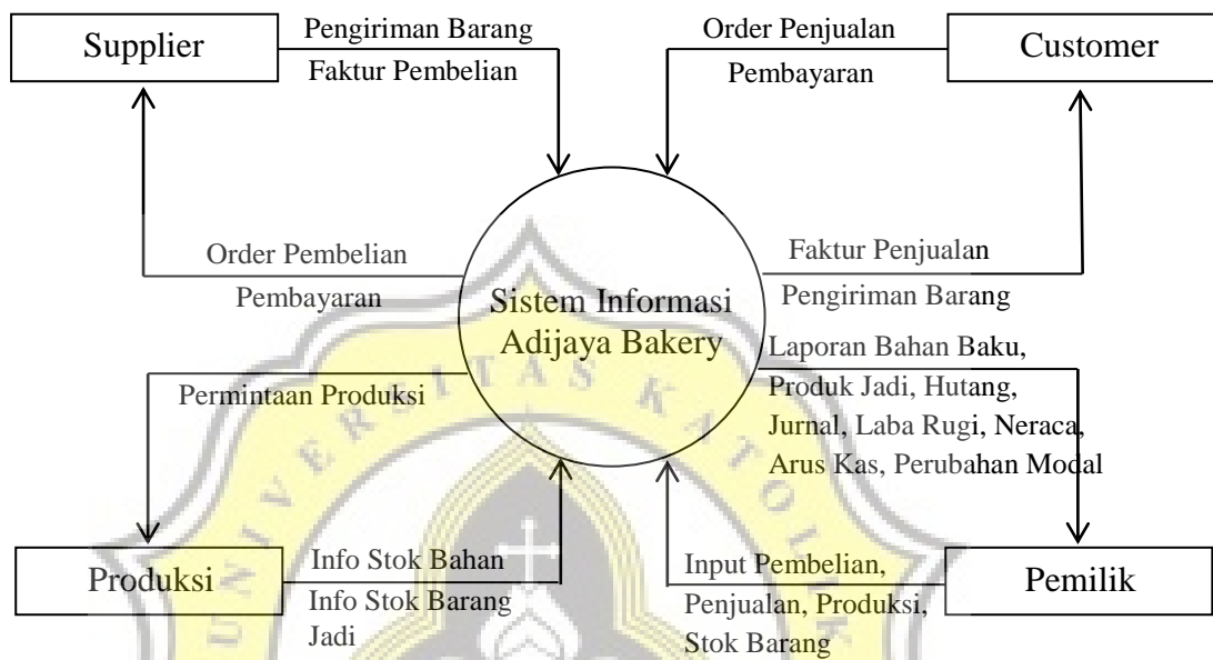
Gambar 4.1 Diagram Konteks Data Flow Diagram (DFD)
