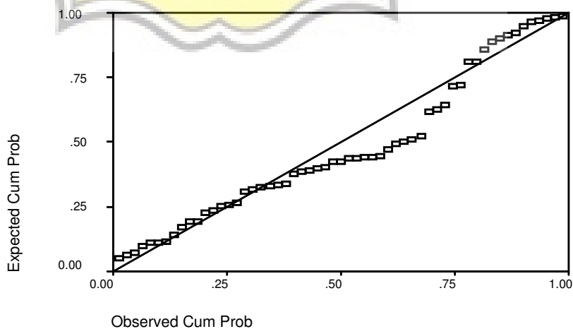
Normal P-P Plot of Regression Standardized Residual Dependent Variable: IKP
