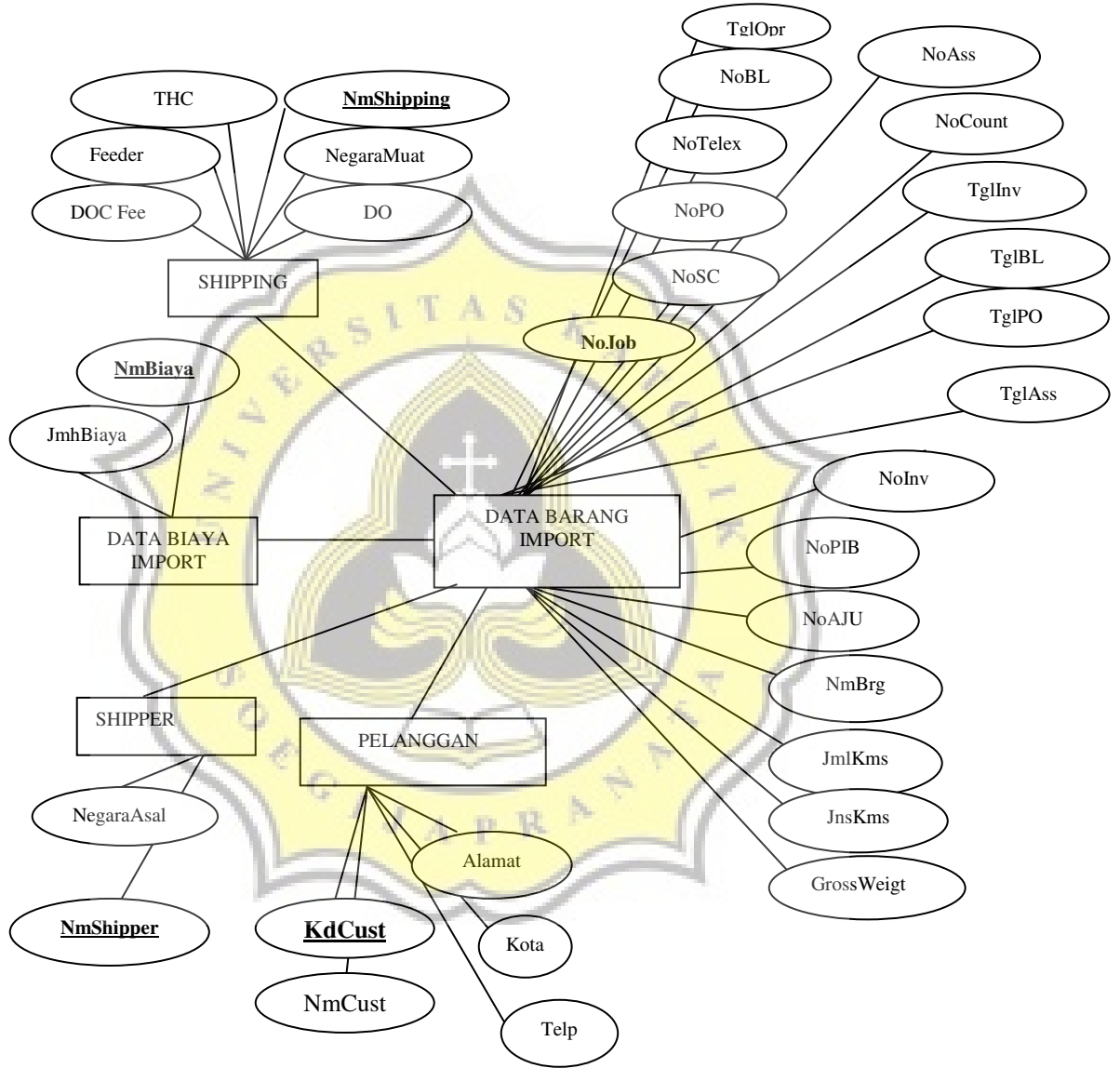
Gambar 4.3 ERD (Entity Relationship Diagram)
