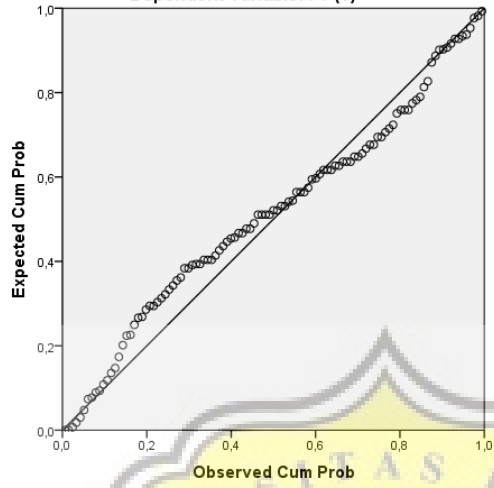
Normal P-P Plot of Regression Standardized Residual Dependent Variable: PP(Y)
