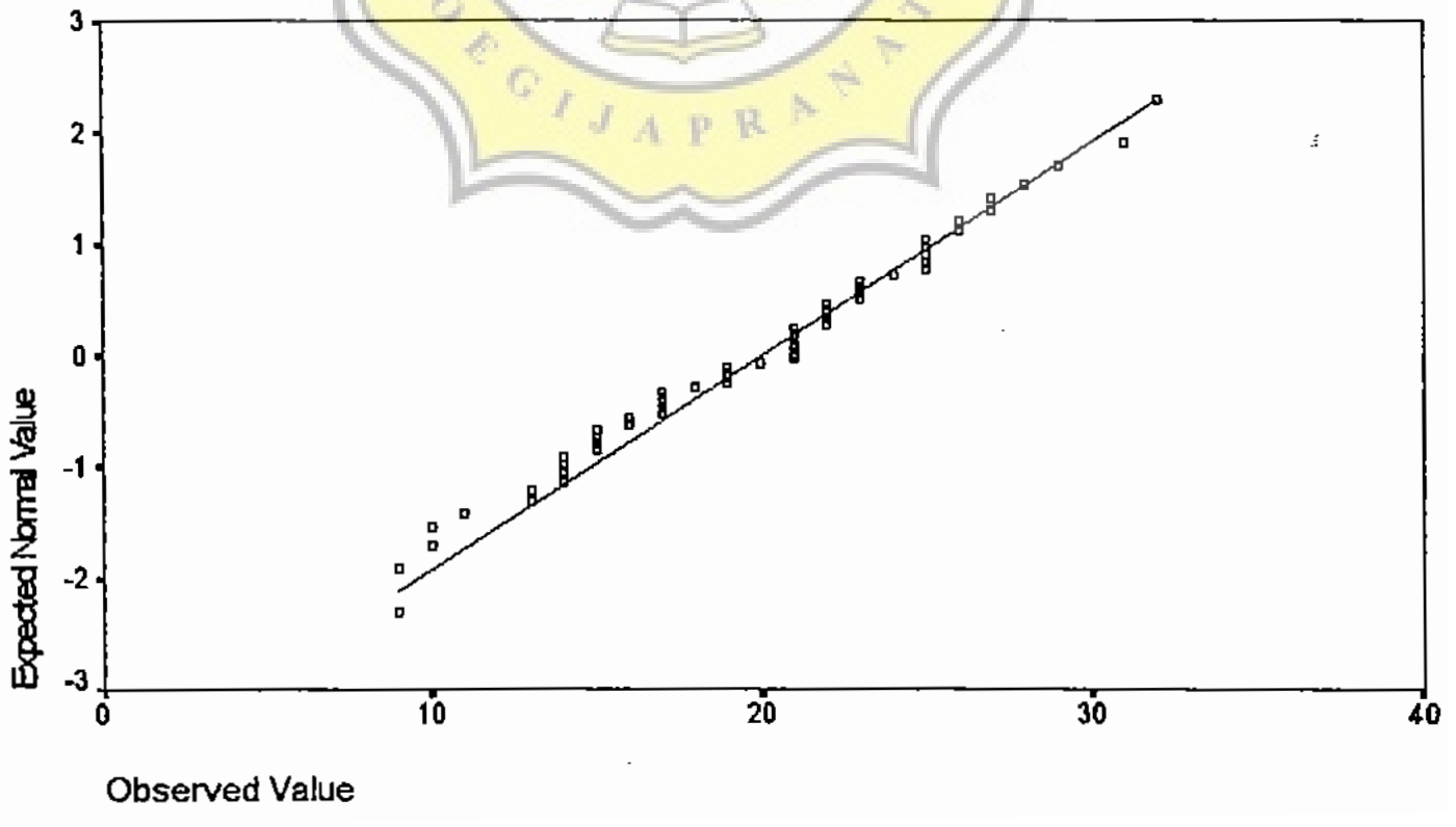
Normal Q-Q Plot of pctotal
