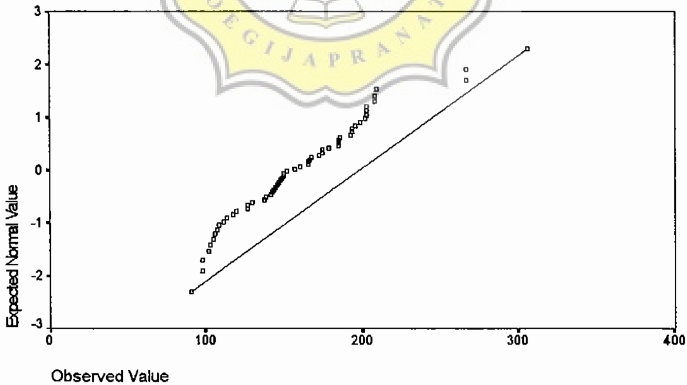
Normal Q-Q Plot of reaksi total
