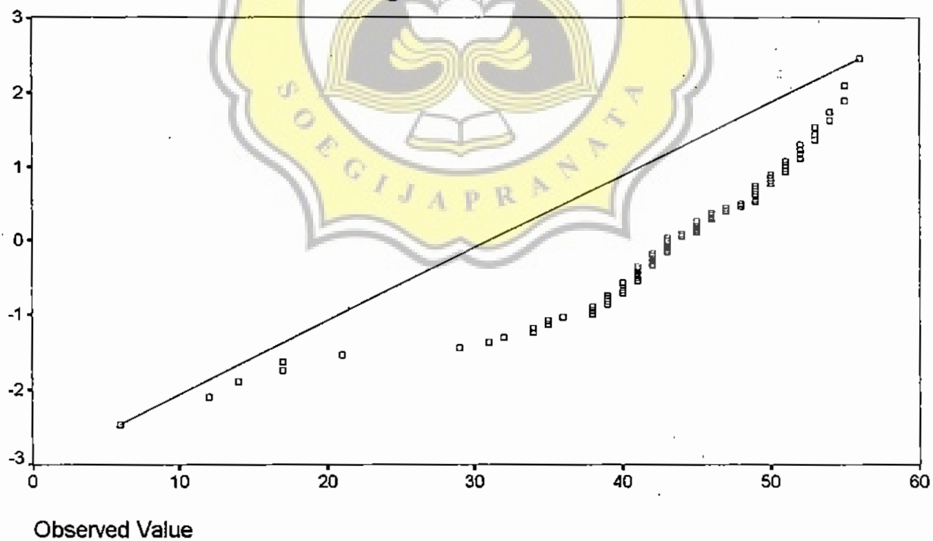
Normal Q-Q Plot of inteligensi
