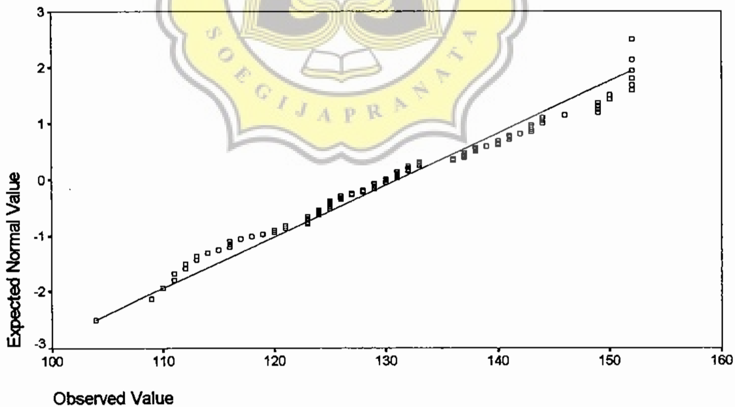
Normal Q-Q Plot of disiplin kerja
