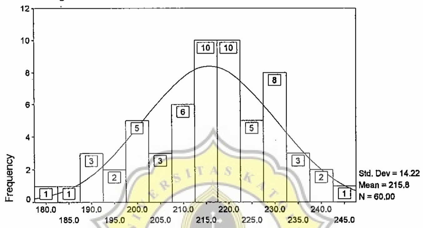
Histogram
