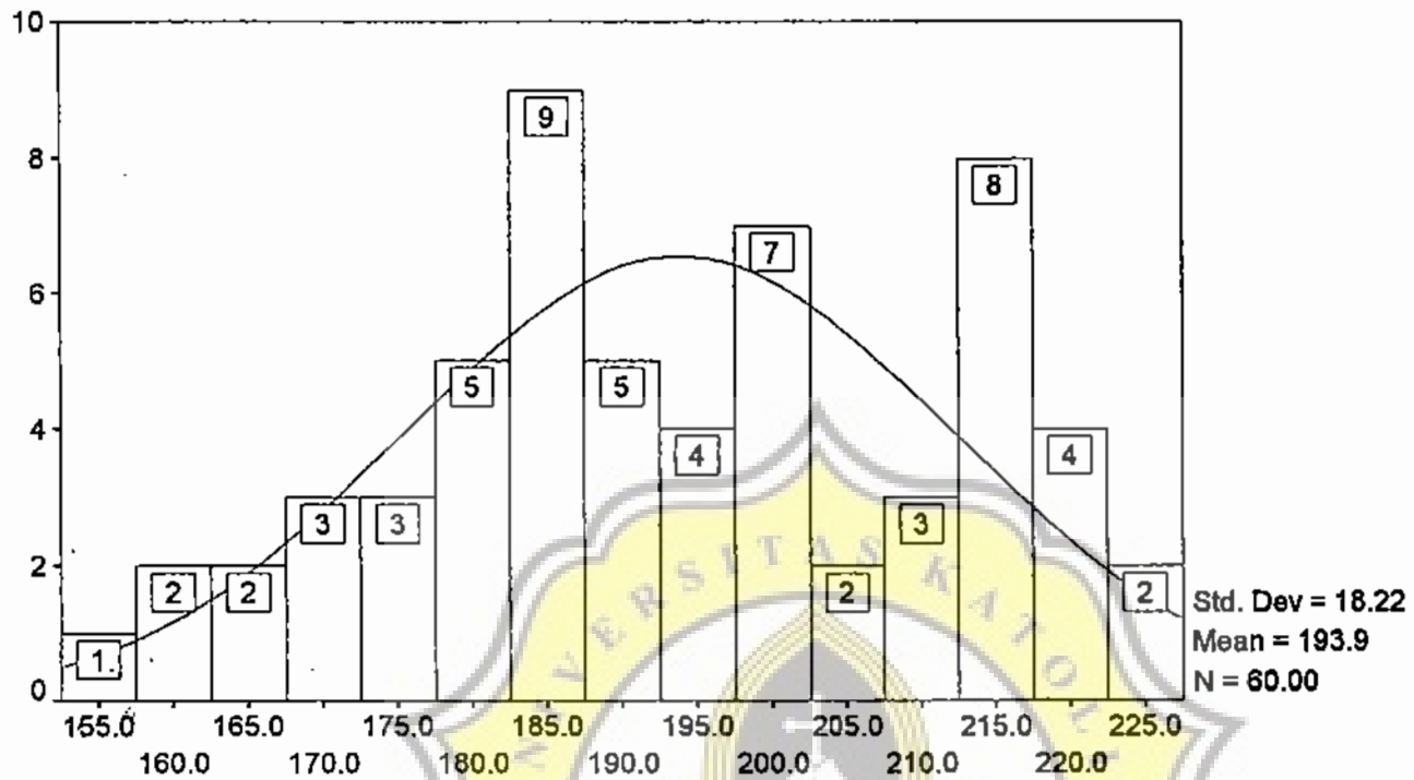
Histogram
